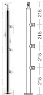
Pipe Type (50ø / 40ø mm)
