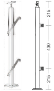
Pipe Type (40 mm x 40 mm)
