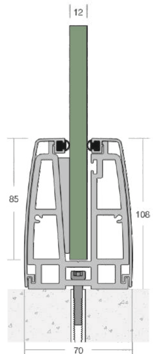
DVH-09 EC SLOTTED
