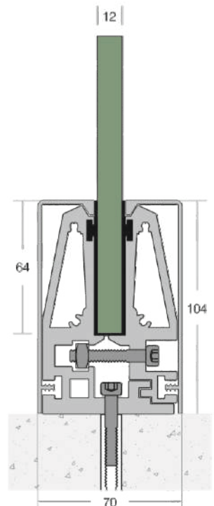
DVH-08B EC SLOTTED
