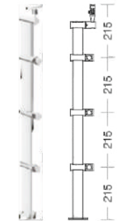
Patta Type (12 mm x 50 mm)
