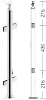
Pipe Type (50ø / 40ø mm)
