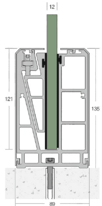
DVH-10 EC SLOTTED
